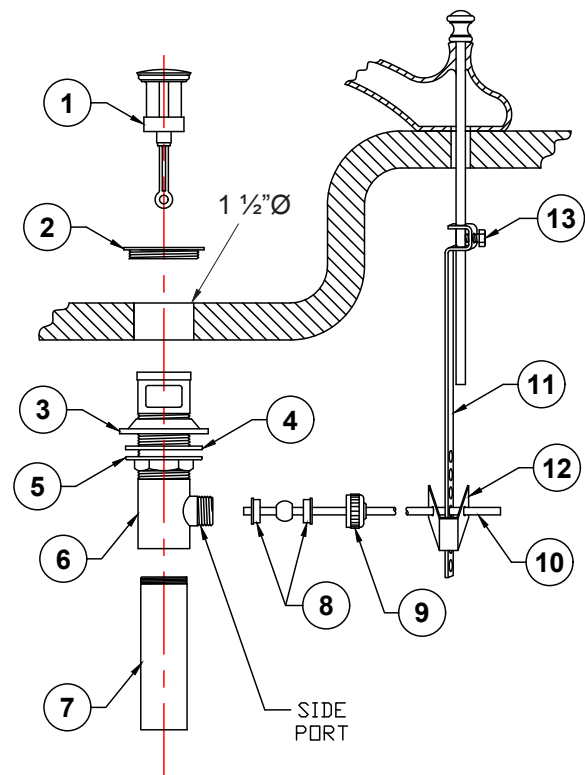
COMPONENT PARTS
