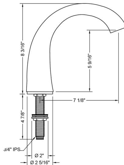
SPOUT-SIDE VIEW
